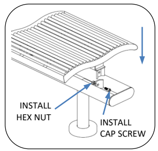
Fig. 3 – Seat install
