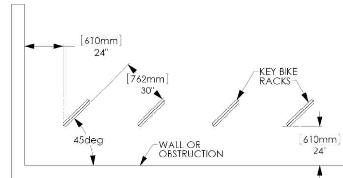
Optional bike rack spacing
