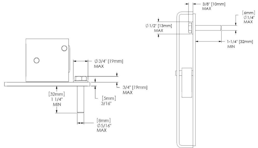
Figure 1 – Surface mount anchor size
