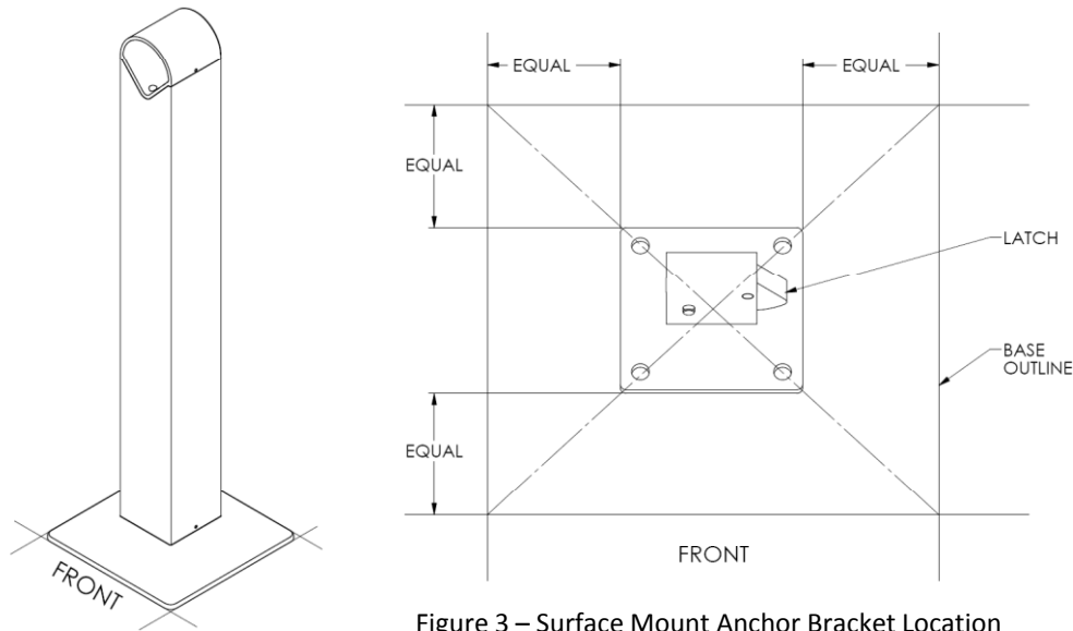
Figure 3 – Surface Mount Anchor Bracket Location
